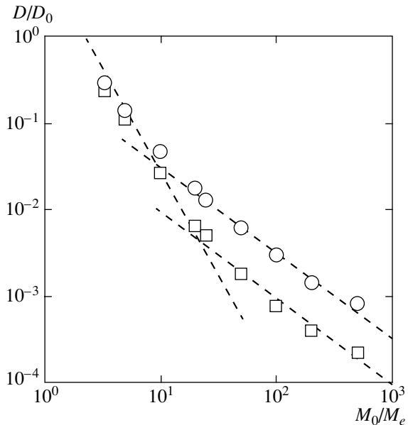
Fig. 3. Self-diffusion coefficient of a macromolecule. Each point shows a value of the ratio of asymptotic values of the displacement of a macromolecule for large times to values of the displacement for the Rouse case of a macromolecule of different lengths among macromolecules with the same lengths. The local anisotropy parameter value is 0.3 for the circles and 0.1 for the squares. The slope of the dashed lines is -2.4 for short macromolecules and -1 for long ones, and hence the simulation gives the well-known dependence D \propto M^{-2} for coefficient of self-diffusion of macromolecules above the point of transition.
