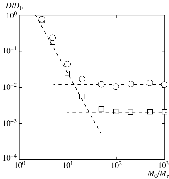
Fig. 2. Diffusion coefficient of a macromolecule. Each point shows a value of the ratio of asymptotic values of the displacement of a macromolecule for large times to values of the displacement for the Rouse case of a macromolecule of length 25M_e among macromolecules with different lengths M_0 . The local anisotropy parameter value is 0.3 for the circles and 0.1 for the squares. The slope of the dashed lines is -2.4 for short macromolecules and 0 for long ones, and hence the simulation determines the point of transition between the diffusive and reptation modes of motion.
