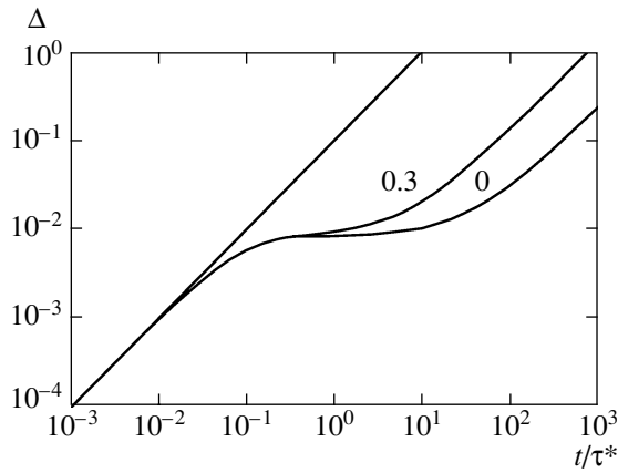
Fig. 1. Displacement of a macromolecule in time. The straight line depicts the analytic result for the Rouse dynamics. The solid curves represent the results for the displacement for a macromolecule of length M = 25M_e among similar macromolecules in accordance with system (1)–(4) with the parameter values B = 429 and \chi = 0.04 . The local anisotropy parameter values a_{ext} are shown at the curves. Internal resistance (parameters E and a_{int} ) does not affect mobility of a macro-molecular coil.
