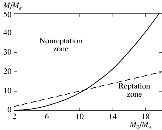
Fig. 4. Alternative modes of motion of a macromolecule. The realization of a certain mode of motion of a macromolecule among other macromolecules depends on the lengths of both the diffusing macromolecule and the macromolecules of the environment. The positions of transition points between two modes are depicted by a solid line. The dashed line marks the systems with macromolecules of equal lengths.
